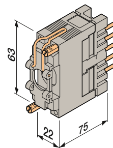
FIM10-1 10 points multicircuits half-base mounting plug
